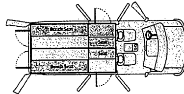
Four (4) Compartment Unit: Model IT-4C (Standard Length) Model IT-4CX (Extended Length) Two Rear & Two Side Inmate Doors
