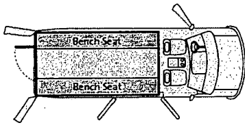
One (1) Compartment Unit: Model IT-1C (Standard Length) Model IT-1CX (Extended Length) One Rear Inmate Door Only.
