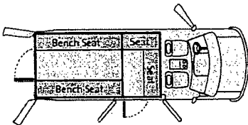
Two (2) Compartment Unit: Model IT-2C-L/R (Standard Length) Model IT-2CX-L/R (Extended Length) One Rear & One Side Inmate Doors.
